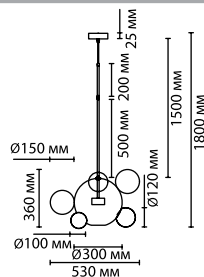
4640/12LB 1 × LED × 12W, 700 lm крепёж: планка
