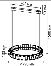
4993/80L 1 × LED × 80W, 2700 lm крепёж: планка
