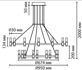
5009/98L 1 × LED × 98W, 2500 lm крепёж: планка
