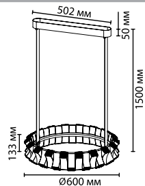
4993/45L 1 × LED × 45W, 1800 lm крепёж: планка
