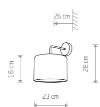
ALICE fabric, painted steel
