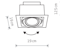
DOWNLIGHT ES111
