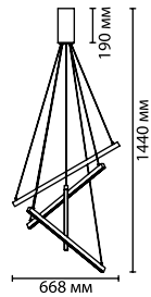
3860/48B 1 × LED × 48W, 2700 lm крепёж: планка
