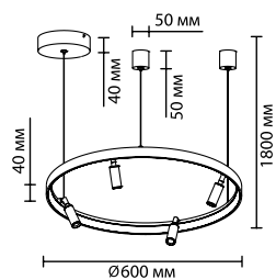
4317/58L 1 × LED × 48W, 4320 lm крепёж: планка
