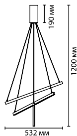
3860/39B 1 × LED × 39W, 2180 lm крепёж: планка
