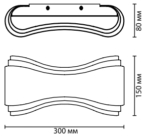
3894/8WS, 3894/8WG 1 × LED × 8W, 257 lm крепёж: планка
