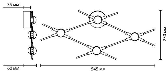
3906/13WL 1 × LED × 13W, 1040 lm крепёж: планка
