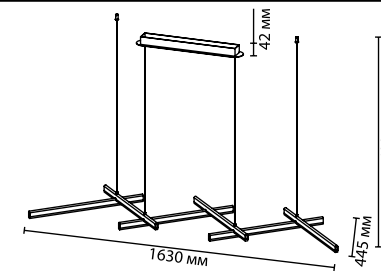
3890/85L 1 × LED × 85W, 4200 lm крепёж: планка
