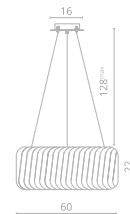
4 7568/02 LM-9 ∅60 | ∅60 | 122 | 128 mm ⚡ 9x60W E14 Ⓜ 15,3
