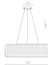
3 7568/02 SP-12 ∅100 | ∅35 | 122 | 128 mm ⚡ 12x60W E14 Ⓜ 18
